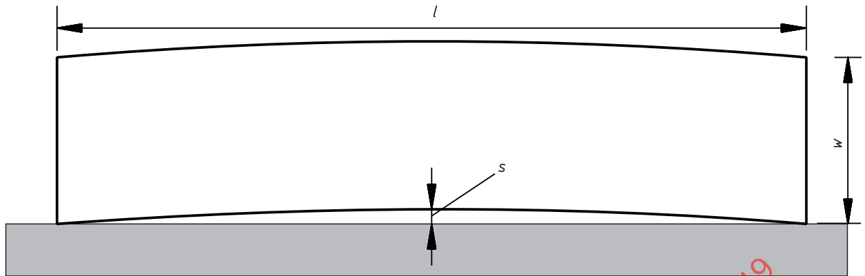
Figure 8 — Determination of straightness s
