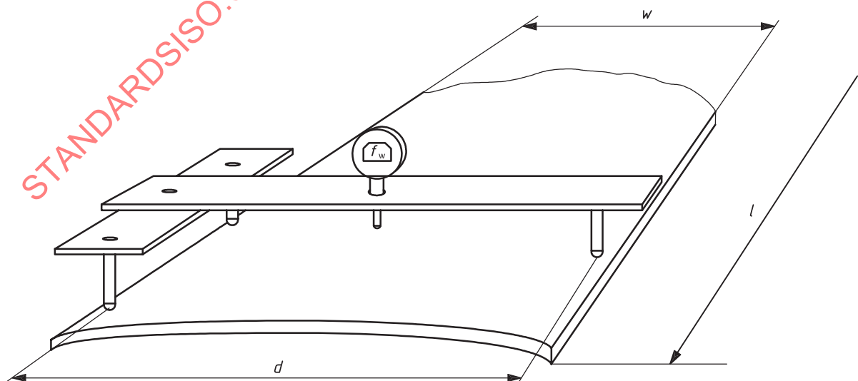
Figure 9 — Determination of width flatness f_w
