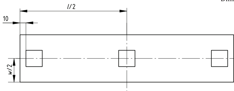
Figure 4 — Sampling from one floor covering element
