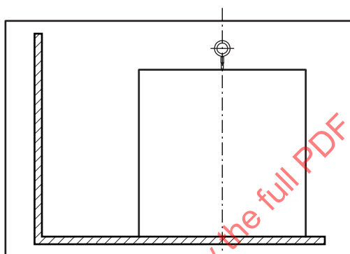
Figure 7 — Apparatus for measuring side length
