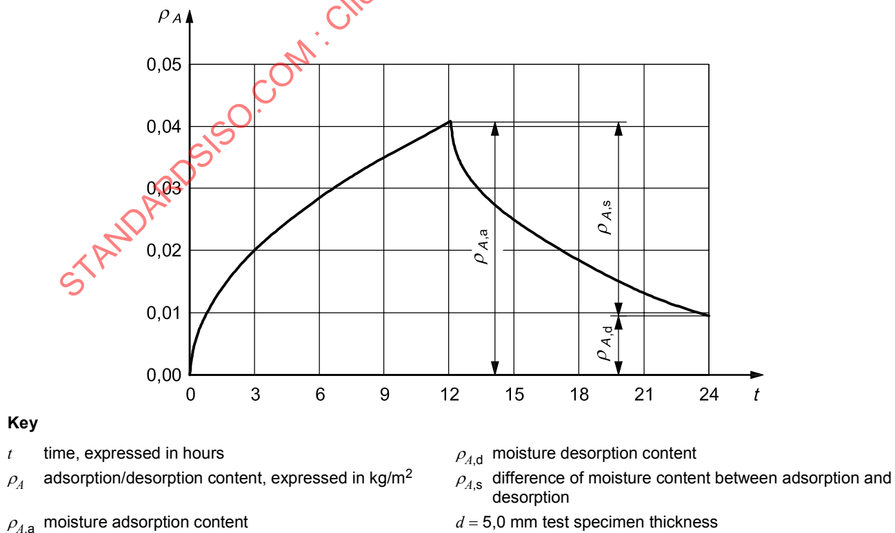
Figure 3 — Typical graph showing moisture adsorption/desorption content over time
