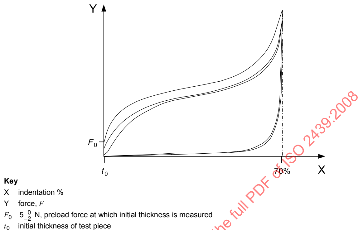
Figure A.1 — Sample force-indentation graph of preliminary indentation, Method A, B or C
