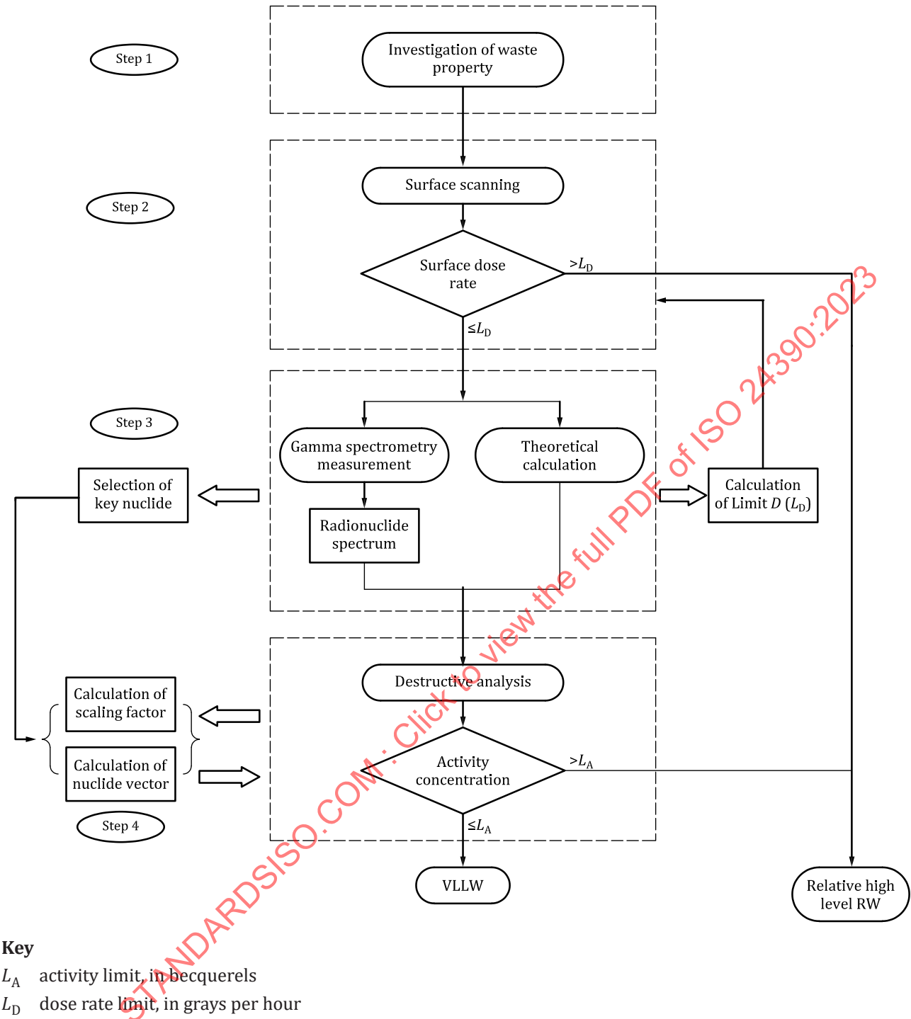
Figure 1 — VLLW radioactivity characterization process
