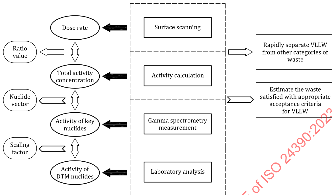
Figure 2 — Correlation of measurement methods for radioactivity characterization of VLLW
