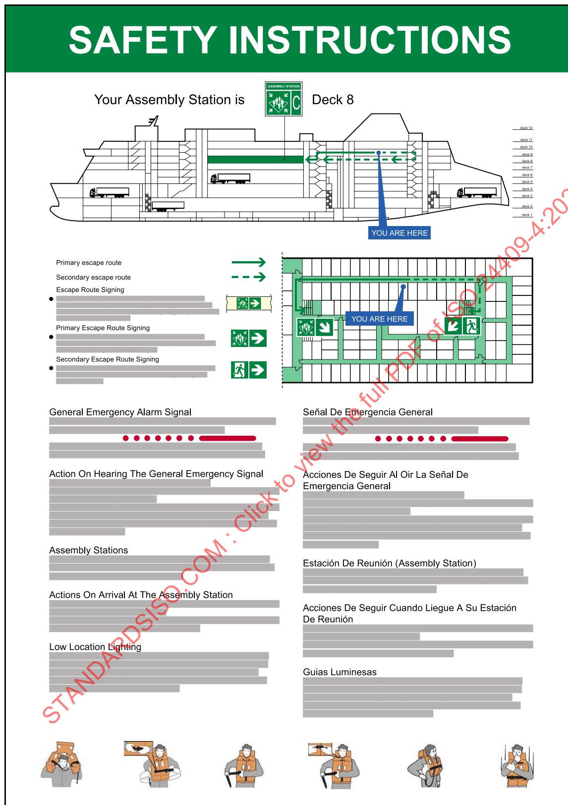
Figure A.1 — Example of a bilingual cabin escape plan sign at a ro-ro ship
