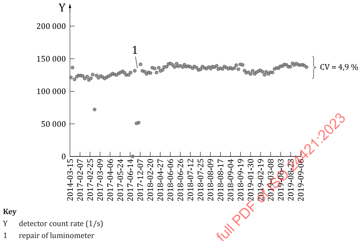
Figure D.1 — Repeated measurements with luminometer using LED reference light source
