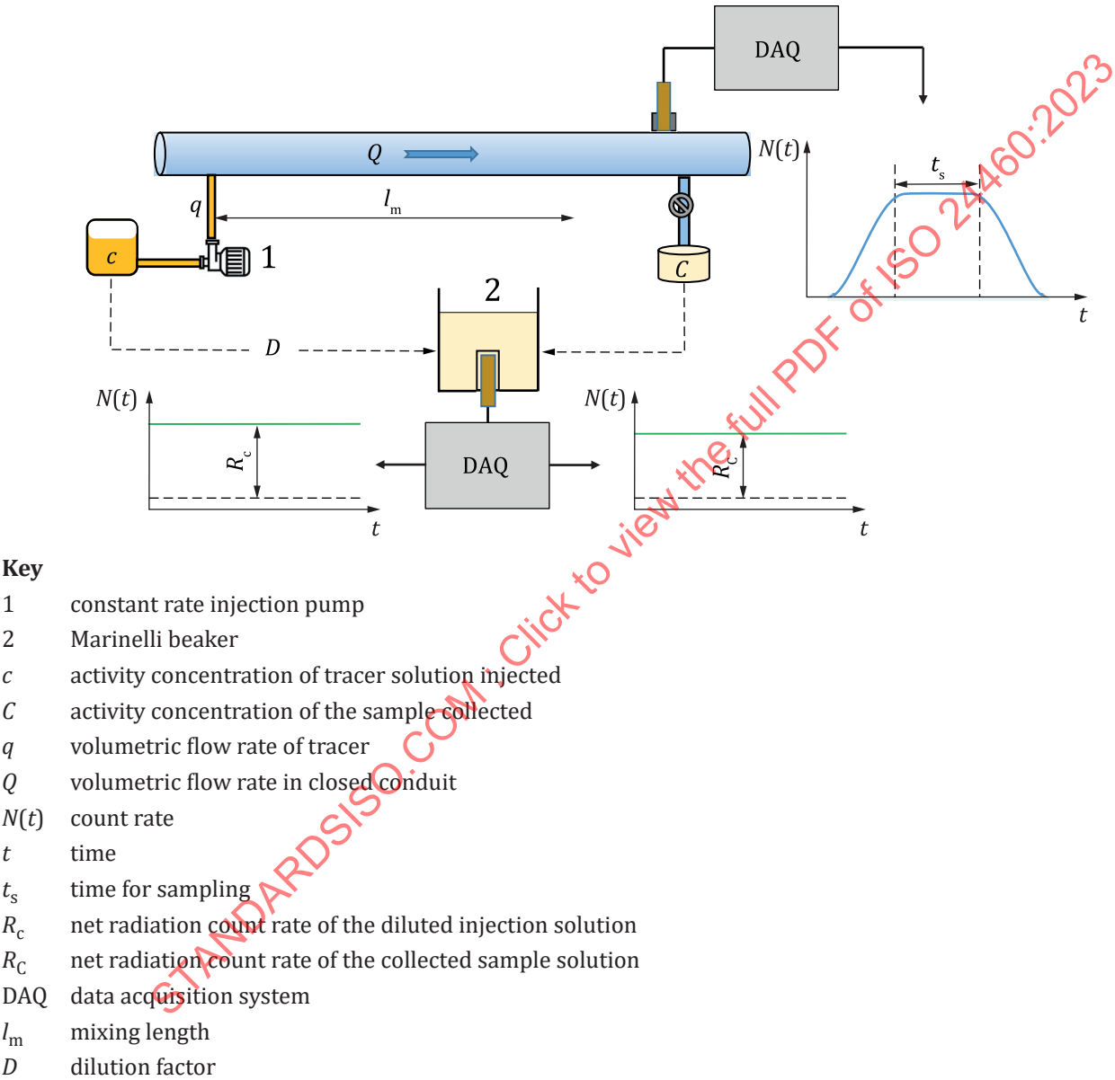
Figure 12 — Flow rate measurement using the constant rate injection method
