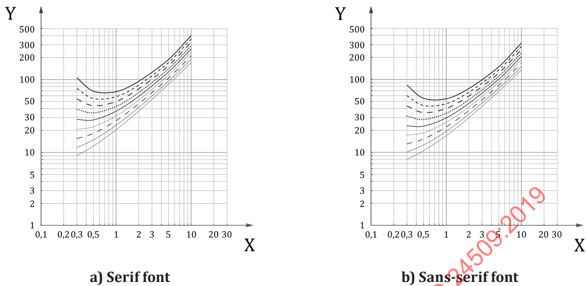
Figure D.5 — Calculated minimum legible font size as a function of viewing distance for different ages from 10 years to 90 years in 10-year steps. Luminance level is 0,1 cd/m 2
