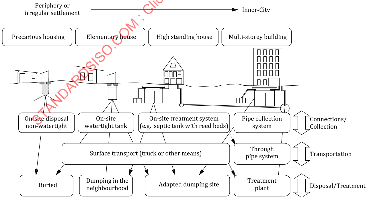
Figure A.1 — Schematic of wastewater systems
