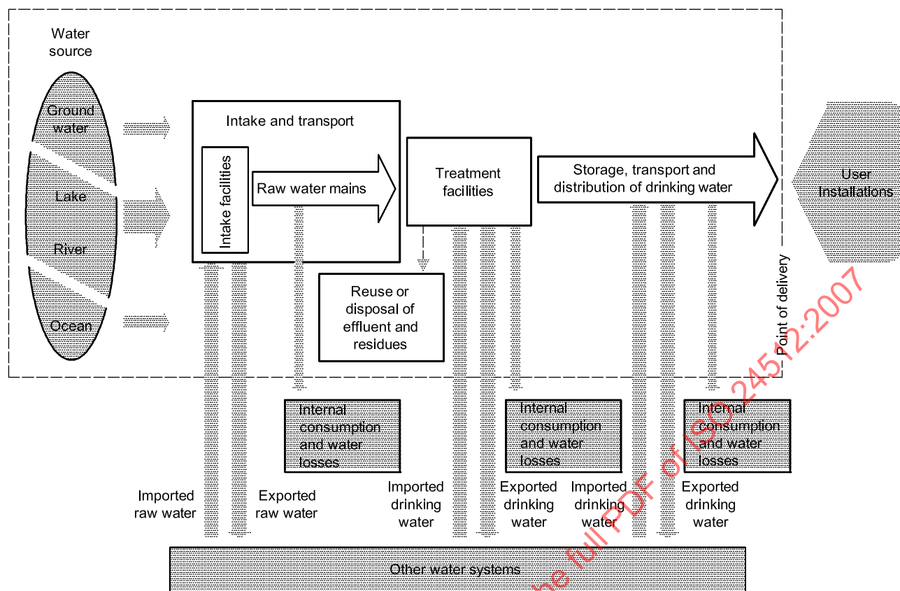
Figure B.2 — Example of a centralized drinking water supply system
