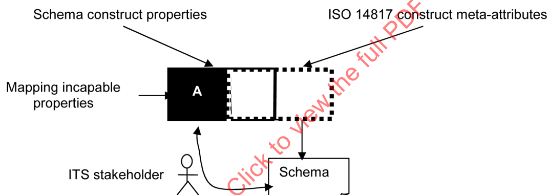
Figure 4 — URL mapping
