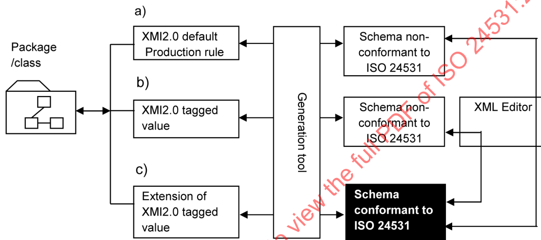
Figure E.2 — UML <-> XML Schema Transformation
