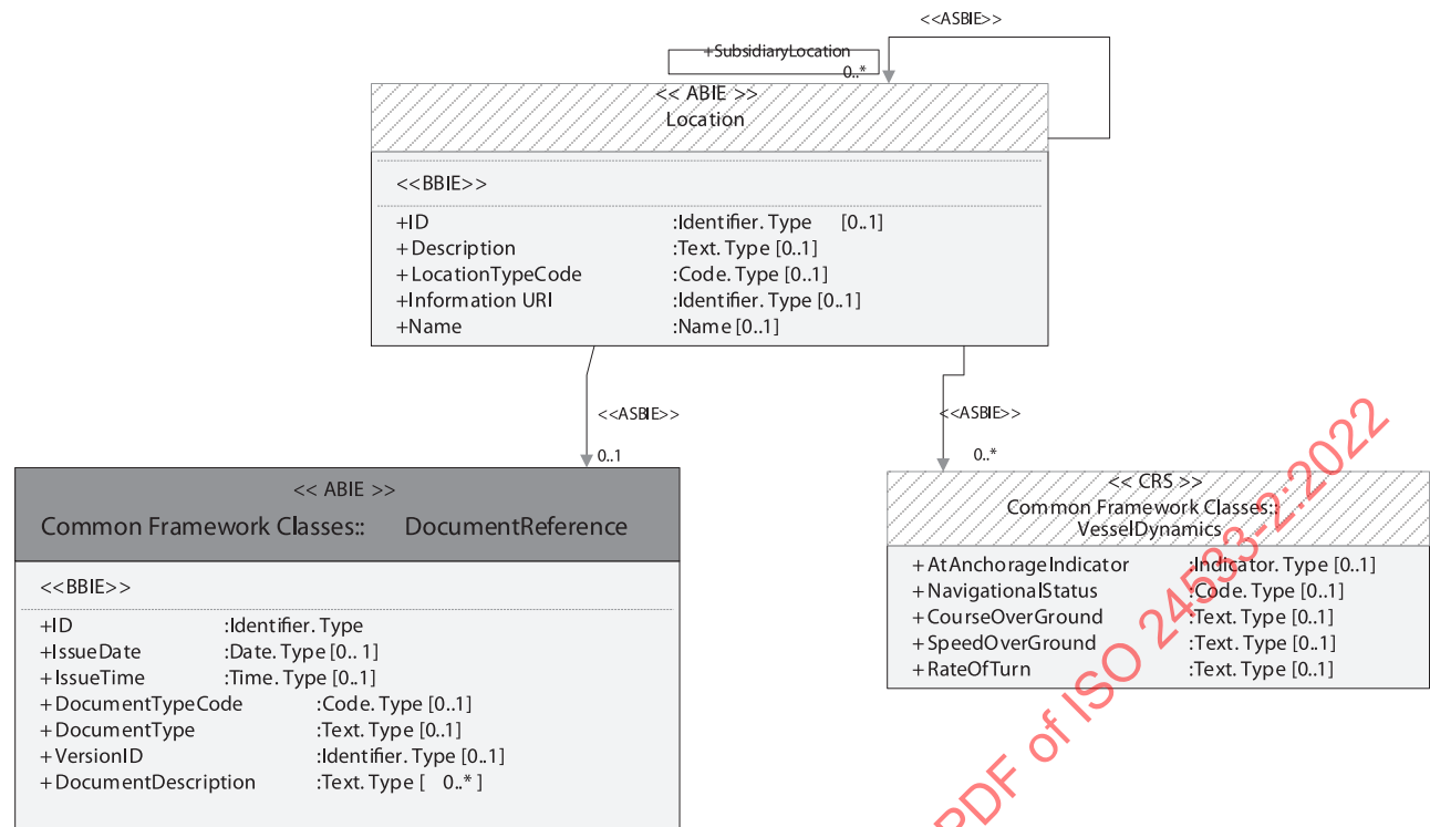
Figure 15 — Location class from UBL
