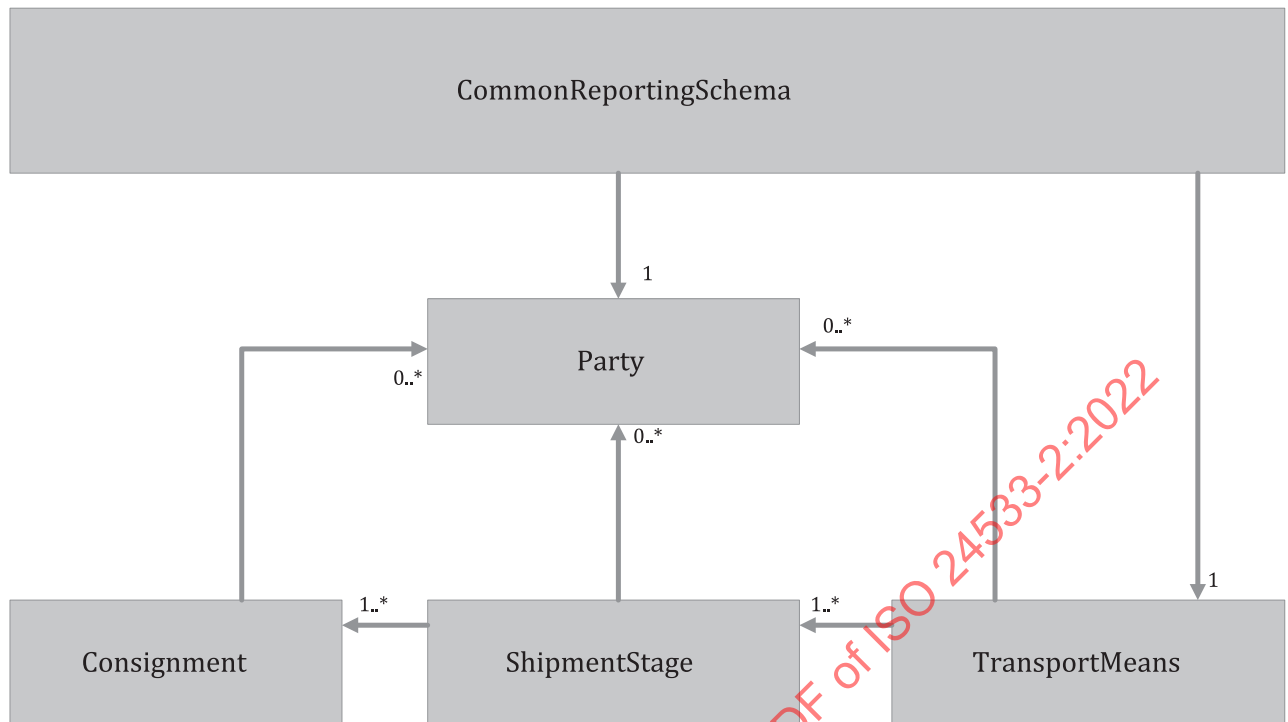
Figure 8 — TransportMeans-oriented CRS structure
