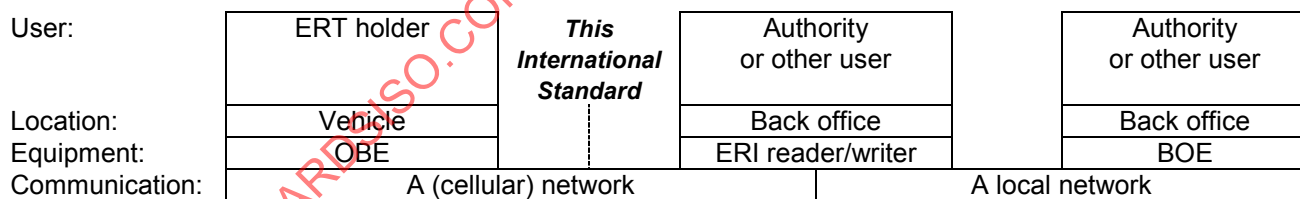
Figure 7 — Overall remote communication concept
