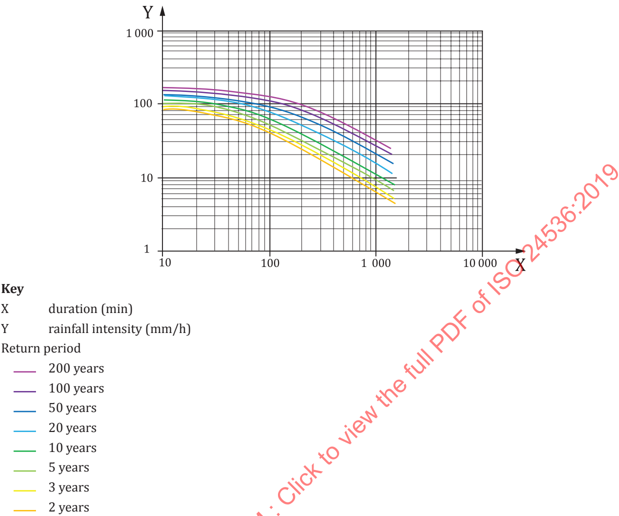
Figure 8 — An example of IDF curves for Hanoi, Vietnam
