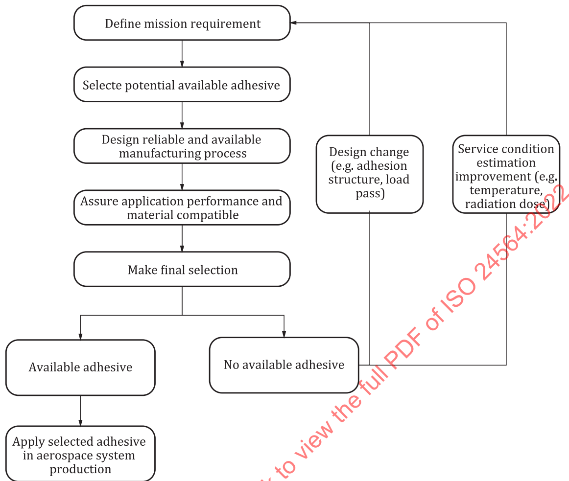
Figure 2 — The procedure of adhesive selection
