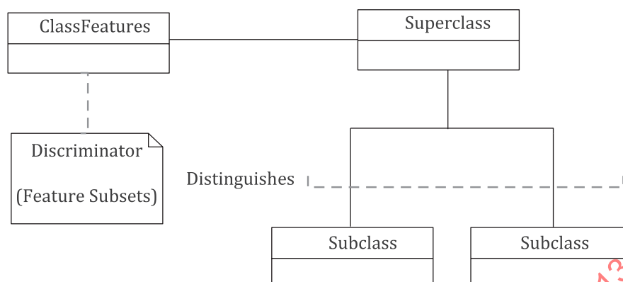
Figure 2 — Methods for data category selection and subclass creation
