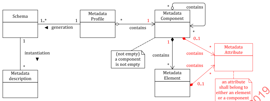
Figure 1 — Component metadata model and its extensions
