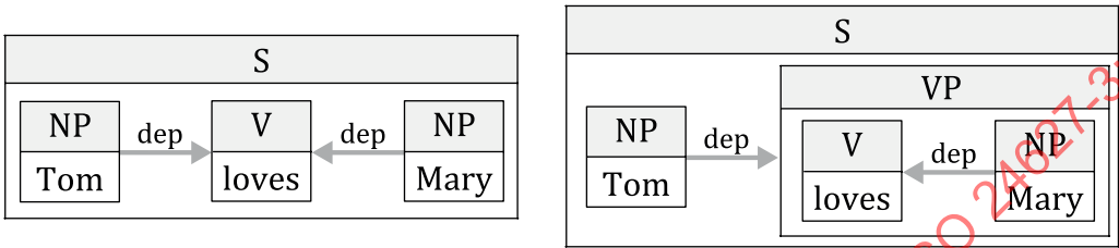
Figure A.7 — Dependency and constituent structures visualized in text segments
