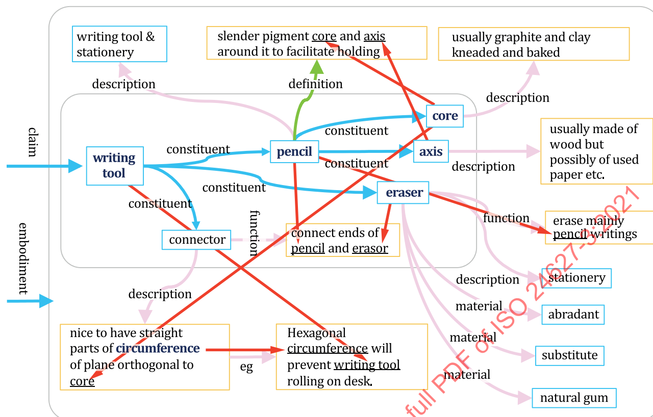
Figure A.2 — Anaphoric links in graph segment
