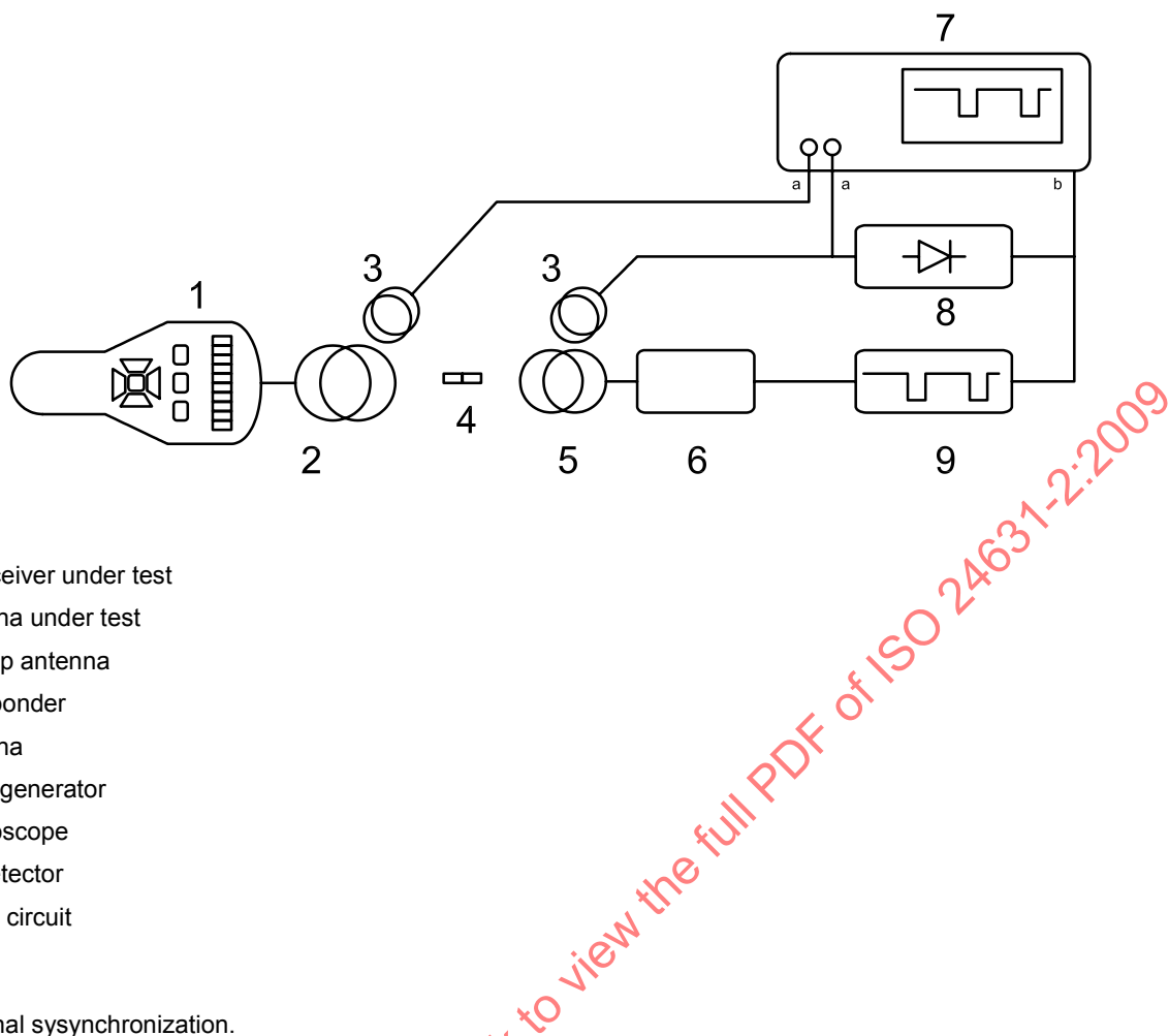
Figure 3 — Test set-up for transceiver activation field timing measurement
