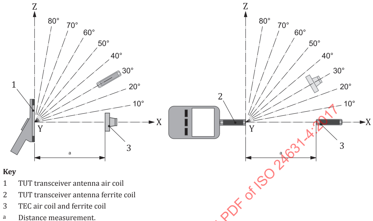
Figure 2 — X-Z measurement plane of transceiver vs. TEC
