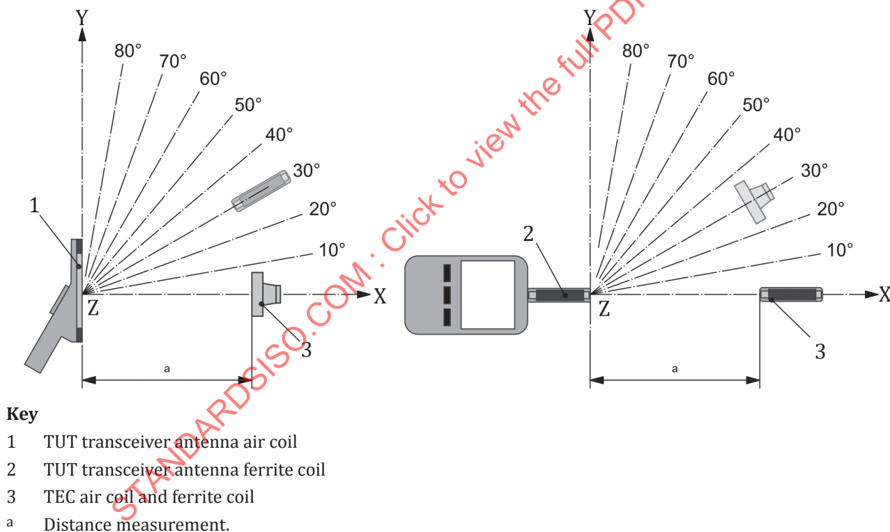
Figure 1 — X-Y measurement plane of transceiver vs. TEC
