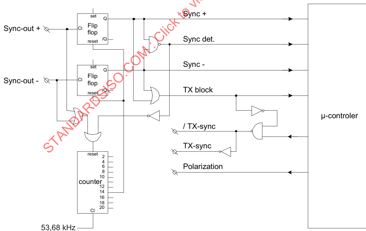
Figure 11 — Synchronization circuit — Logic block
