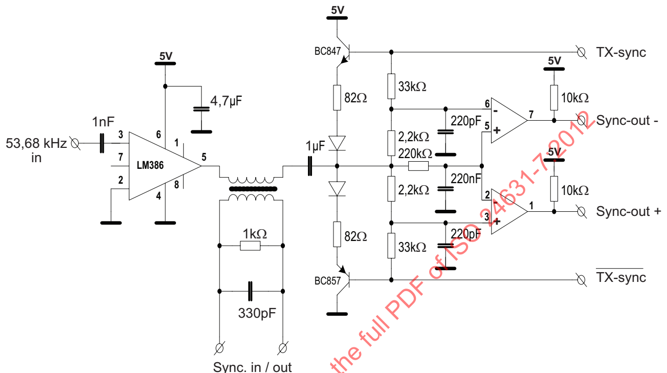
Figure 12 — Synchronization circuit — Sync detector
