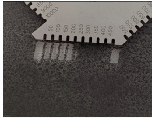
b) Film thickness gauge
