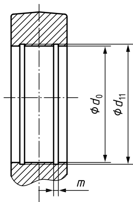
Figure B.4 — Retaining ring groove
