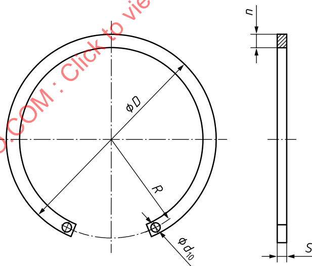
Figure B.3 — Retaining ring with clamp holes d_0 > 200 mm
