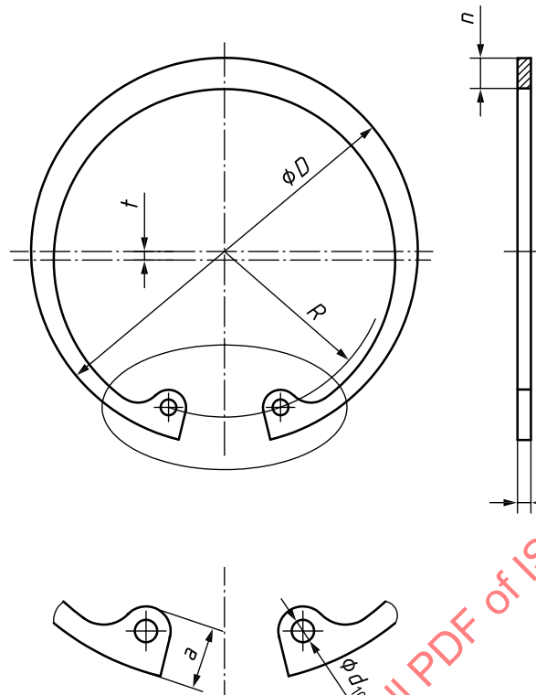
Figure B.2 — Retaining ring with clamp holes d_0 \leq 200 mm
