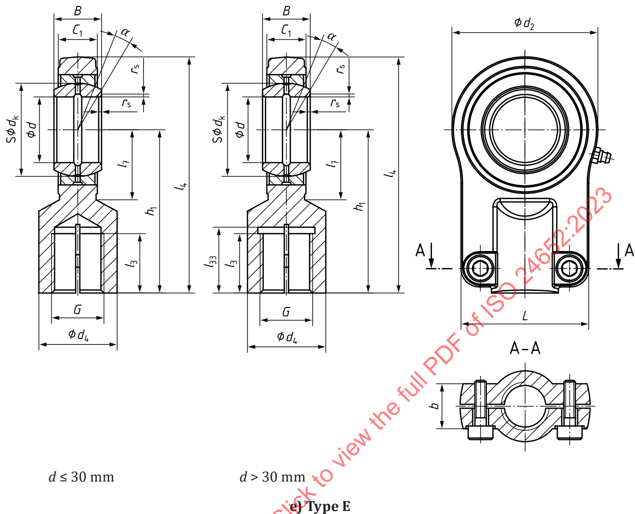
Figure 3 — Spherical plain bearings rod end, threaded type
