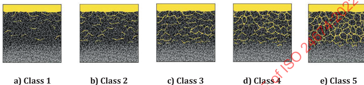
Figure 2 — Pictorial representations of the classes defined in Table 3
