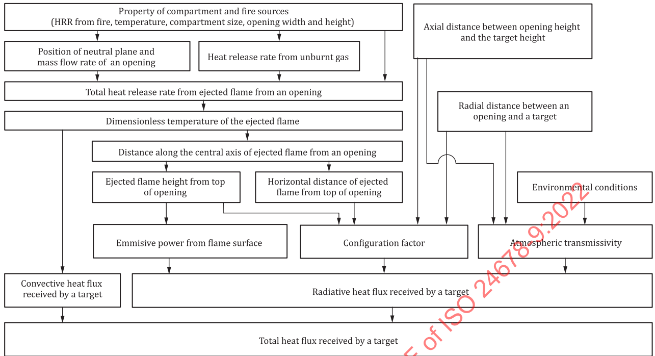
Figure A.2 — Calculation process of heat flux received by a target from an ejected flame
