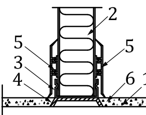
e) Lining to deck
