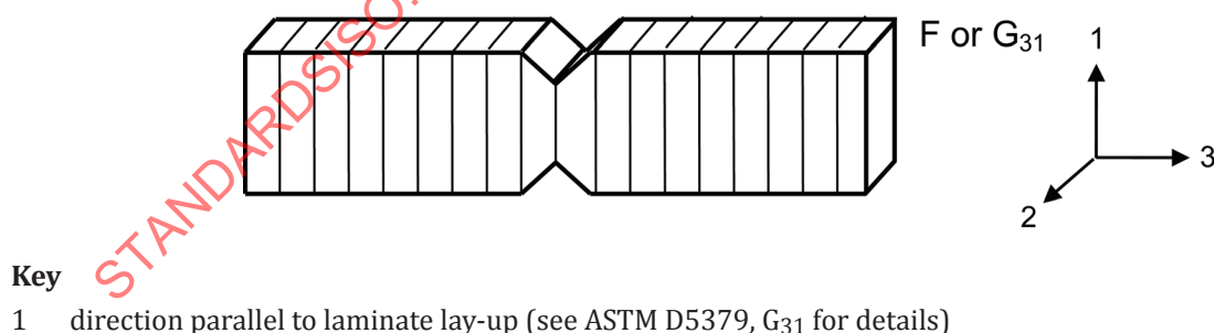
Figure B.1 — Test specimen geometry from ASTM D5379
