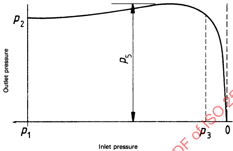
Figure 5 — Dynamic expansion curve with rising characteristic and maximum
