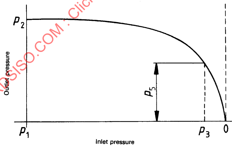
Figure 6 — Dynamic expansion curve with falling characteristic
