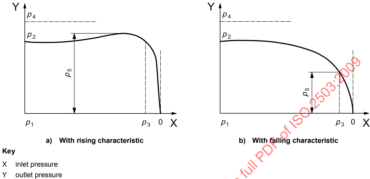
Figure 2 — Typical dynamic expansion curves
