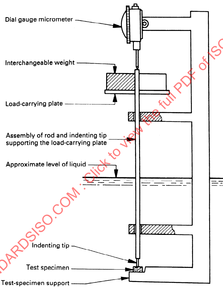
Figure 1 — Apparatus for determining the Vicat softening temperature
