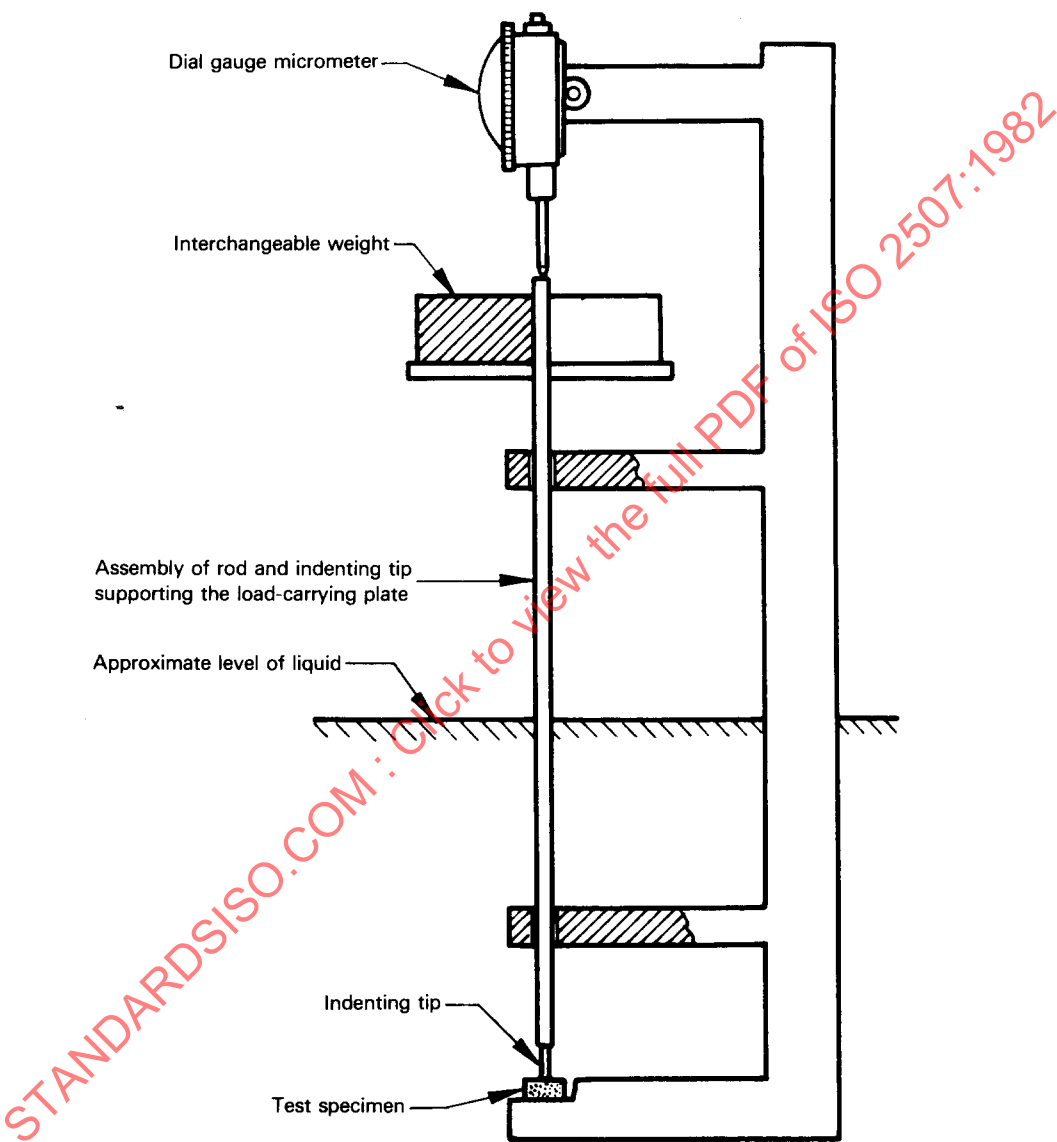
Figure — Schematic diagram of apparatus for the determination of the Vicat softening temperature
