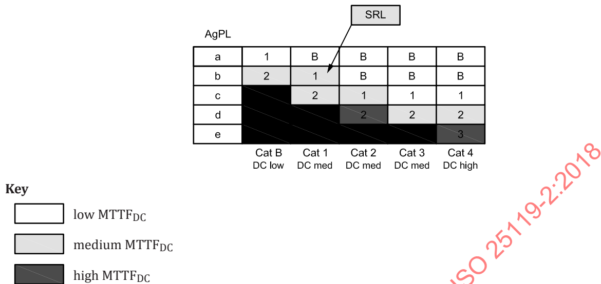
Figure 2 — Relationship between AgPL, categories, MTTF DC , DC and SRL
