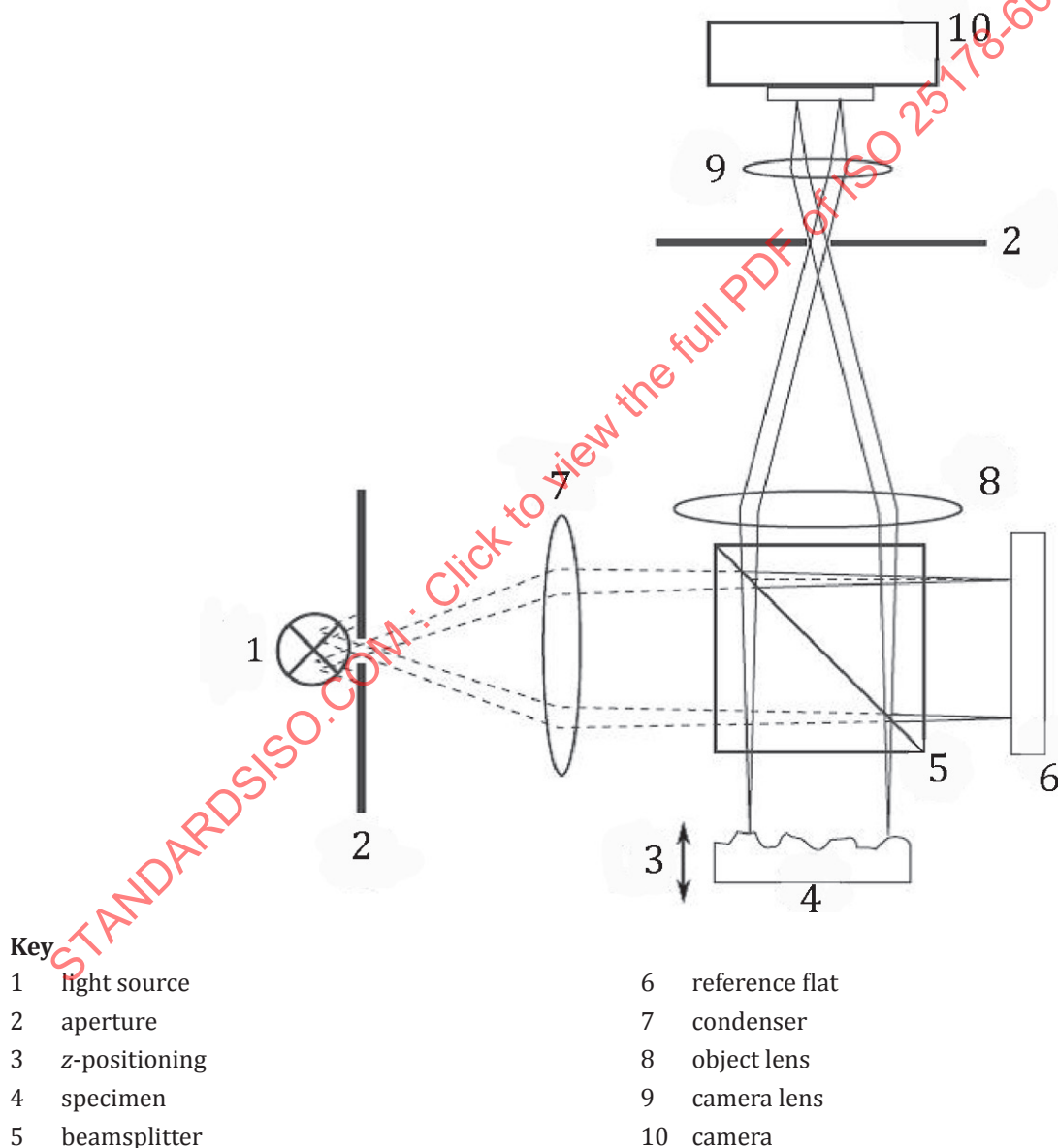
Figure A.2 — Optical principle of a Twyman-Green-interferometer with camera sensor
