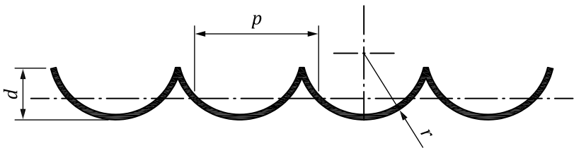
Figure 4 — Arcuate shape
