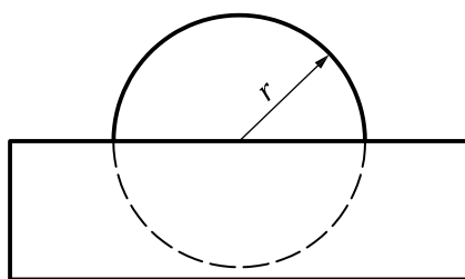
Figure 18 — Hemisphere standard
