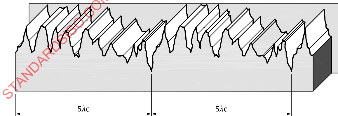
Figure 9 — Irregular profile standard
