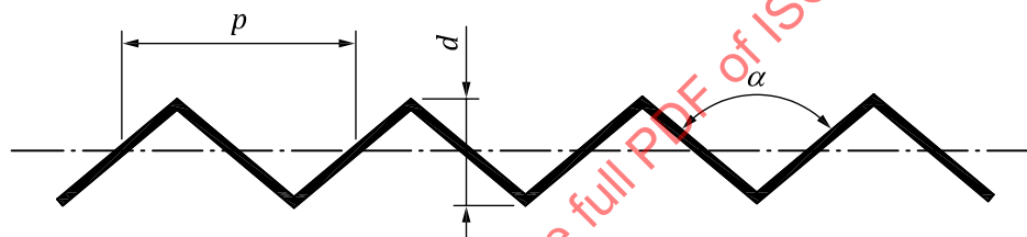
Figure 2 — Triangular shape
