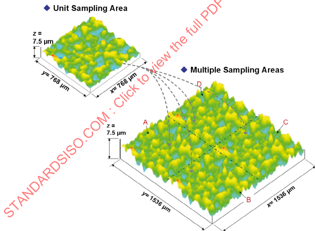
Figure 24 — Areal irregular material measure
