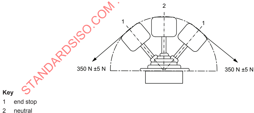
Figure 2 — Extreme-travel test, X and Y movements
