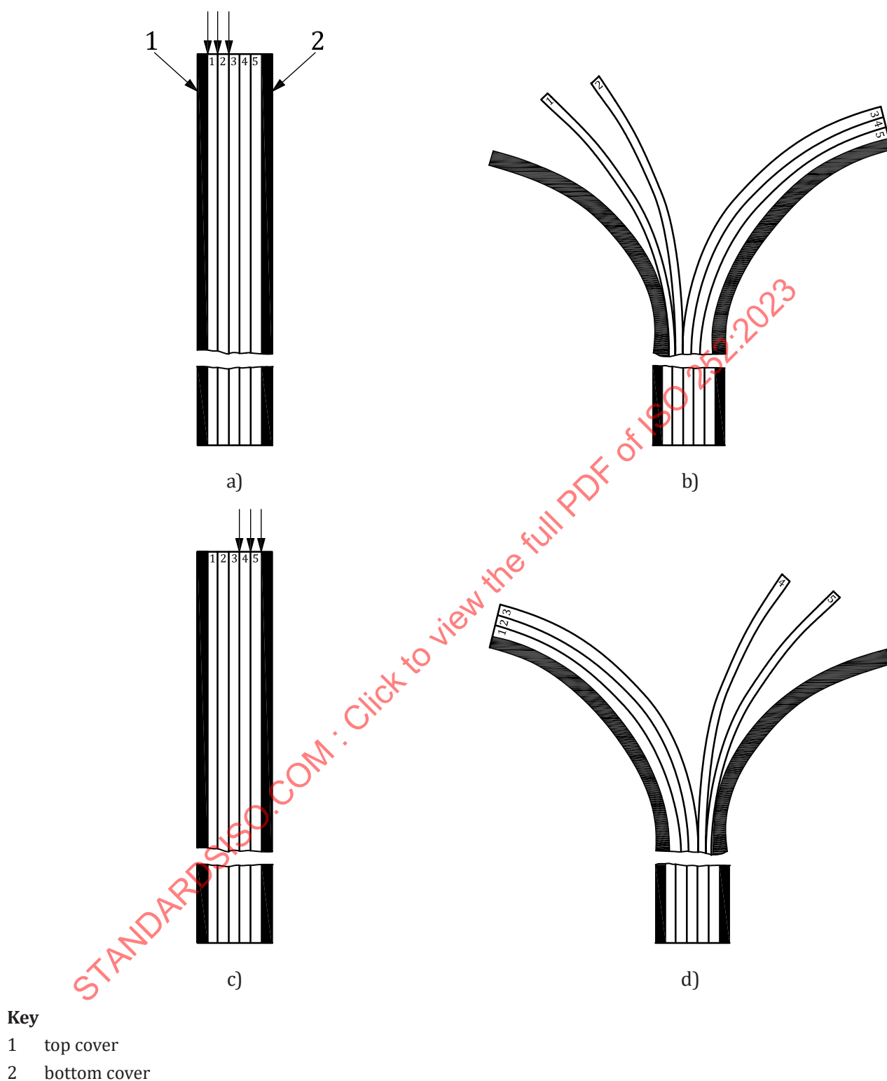
Figure 1 — Sequence of separation of components for method A (5-ply belt shown as example)
