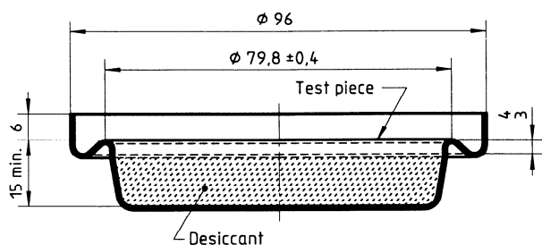
Deep dish (5.1) for materials with transmission rate greater than 100 \text{ g}/(\text{m}^2 \cdot \text{d}) , (tapered to nest)
