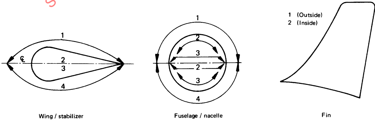
FIGURE 1 — Examples of use of the fourth digit (work locator)
