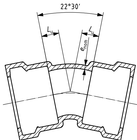
Figure 10 — Double-socket 22° 30' bend
