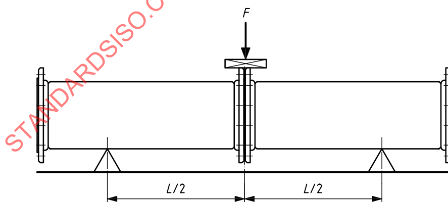
Figure 3 — Strength and leaktightness test for flanged joints
