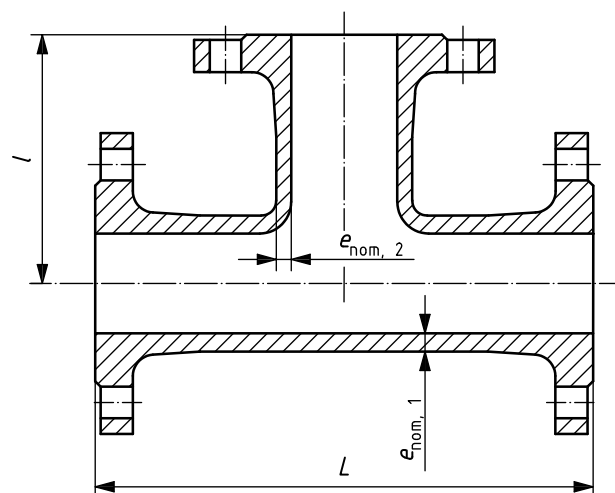
Figure 18 — All flanged tee
