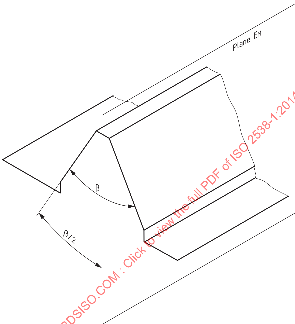
Figure 3 —Vee-block
