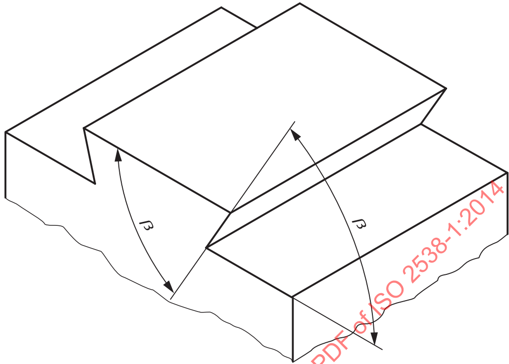
Figure 2 — Dovetail
