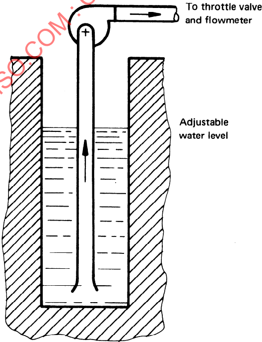
FIGURE 7 — Cavitation tests — Variation of (NPSH) by control of liquid level at inlet (see Figures 1 and 2)
