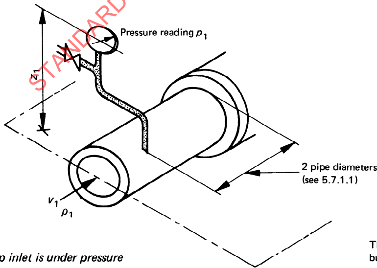
FIGURE 2 – Test of a centrifugal pump by means of Bourdon gauges
