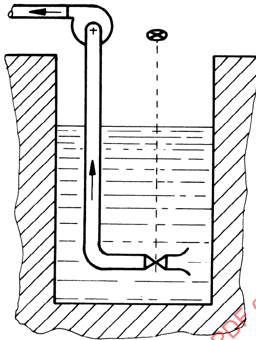
FIGURE 8 — Cavitation tests — Variation of (NPSH) by means of a throttle valve at inlet (see Figures 1 and 2)
