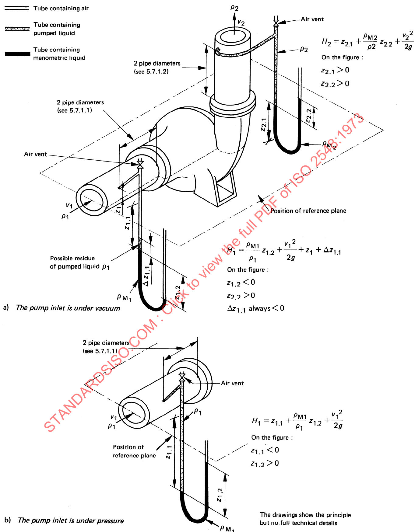
FIGURE 1 — Test of a centrifugal pump by means of liquid column gauges
