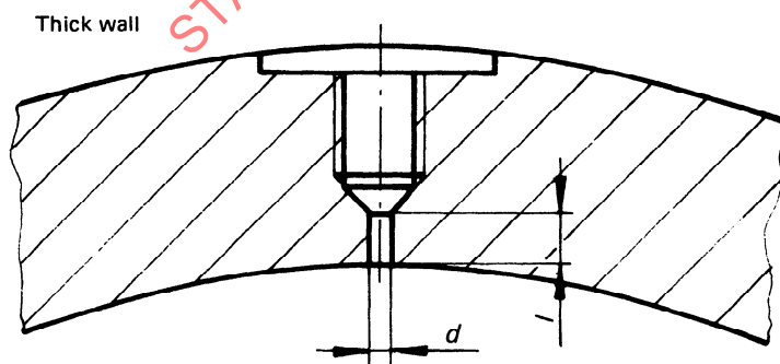
FIGURE 4 — Requirements for static head tapings
