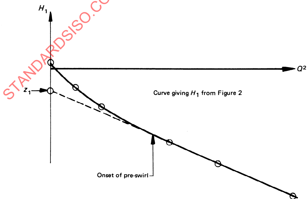
FIGURE 12 — Correction of measured inlet head
