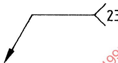
Figure 11 — Indication of welding process
