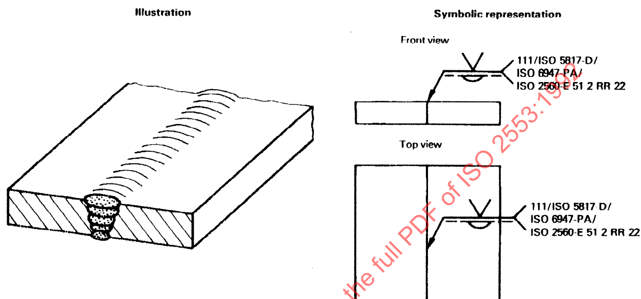
Figure 13 — Single-V butt weld with backing run
