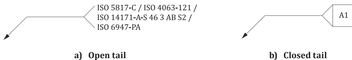
Figure 6 — Examples of the use of a tail on welding symbols
