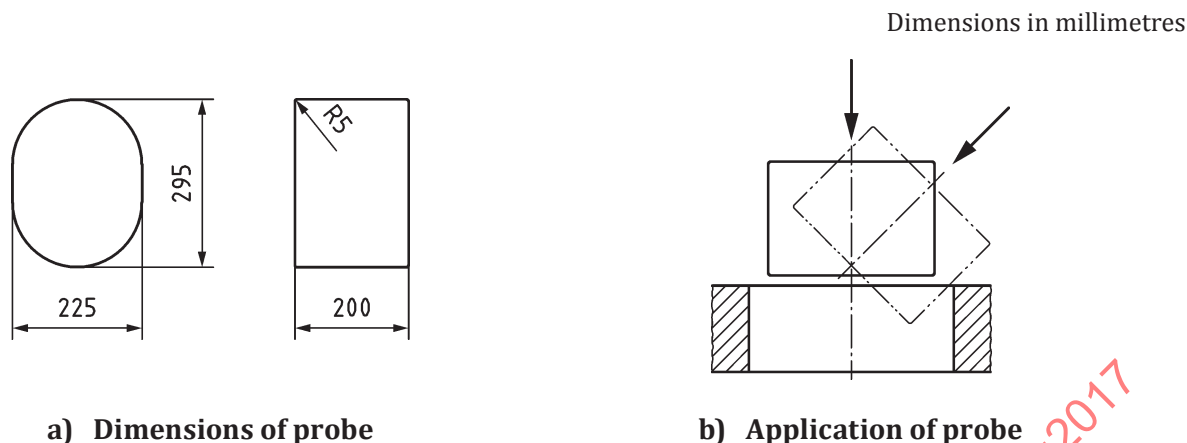
Figure 3 — Child torso probe, 10 years of age
