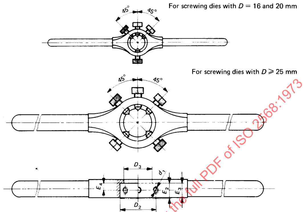
FIGURE 3 – Die stocks
