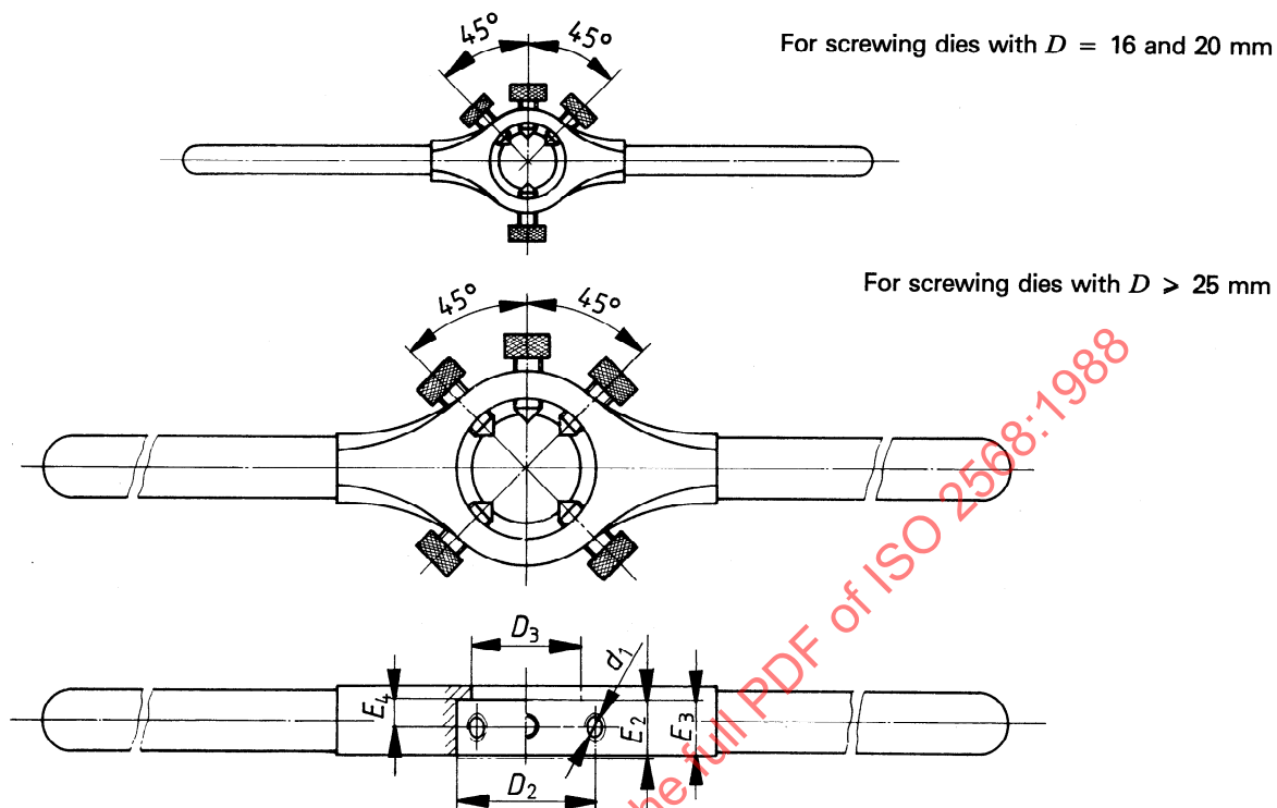
Figure 3 — Die stocks
