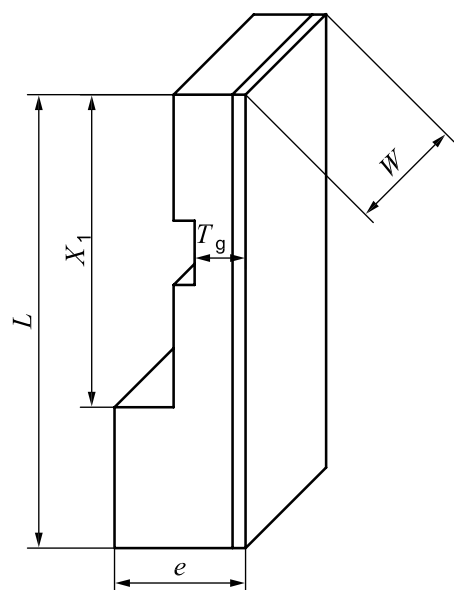
a) Rebated and grooved test-piece
