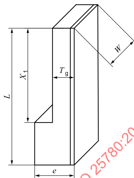
b) Rebated test-piece
