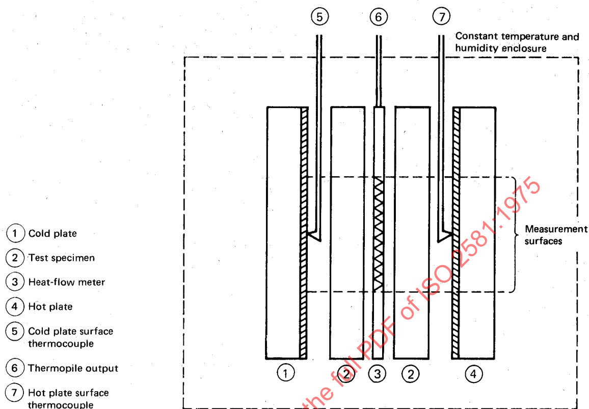
FIGURE 1 — Heat-flow meter apparatus with two test specimens (method S)
