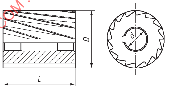
Figure 1 — Solid cutters
