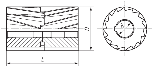
Figure 2 — Interlocking cutters
